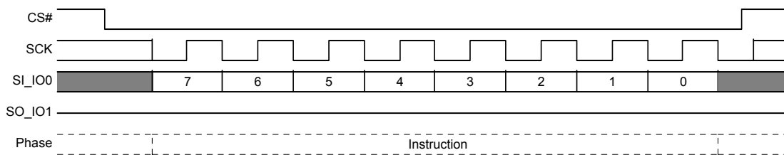
Figure 63. Enter QPI Mode (QPIEN 38h) Command Sequence
